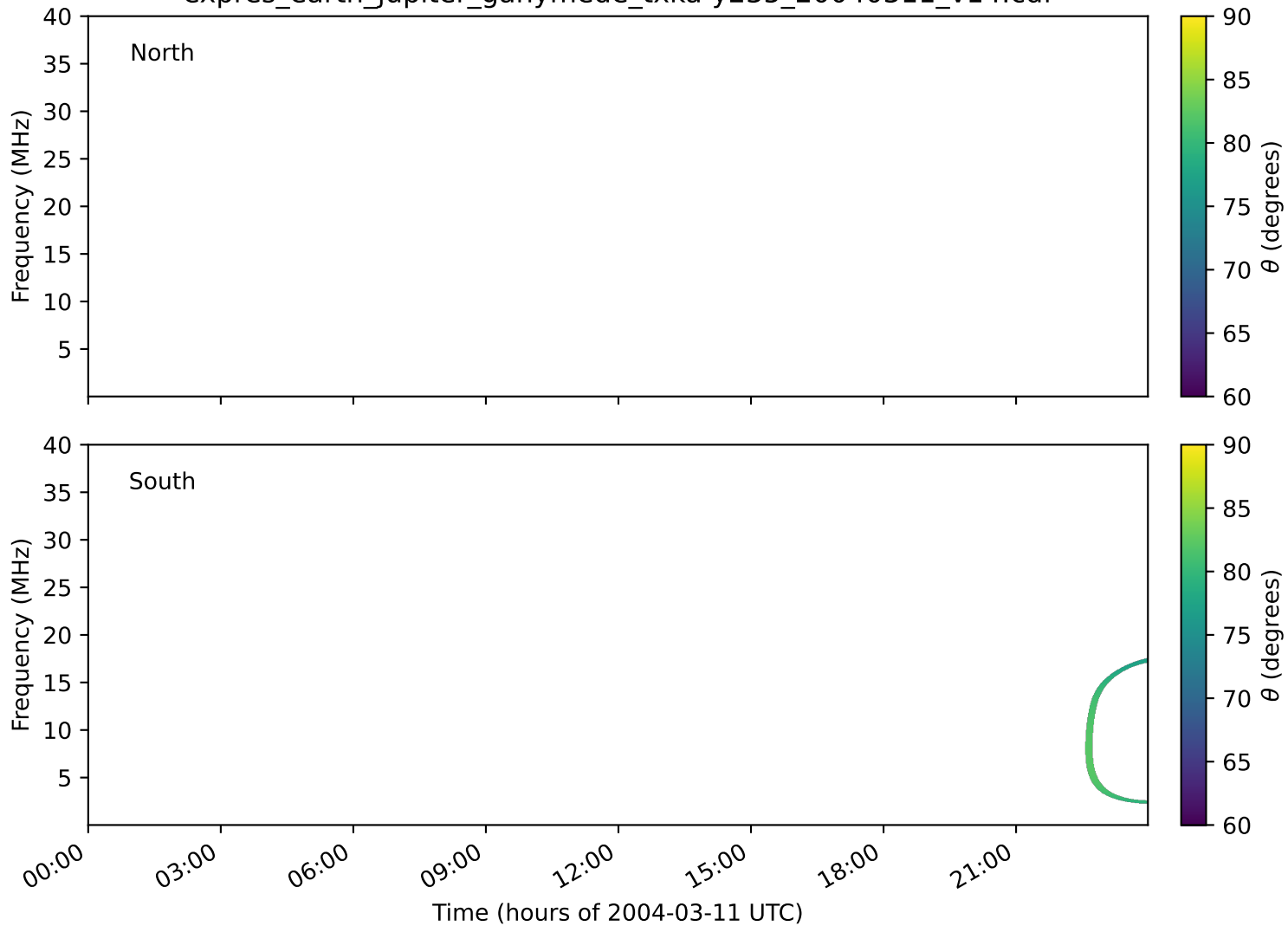
expres_earth_jupiter_ganymede_txka-y235_20040311_v14.cdf
