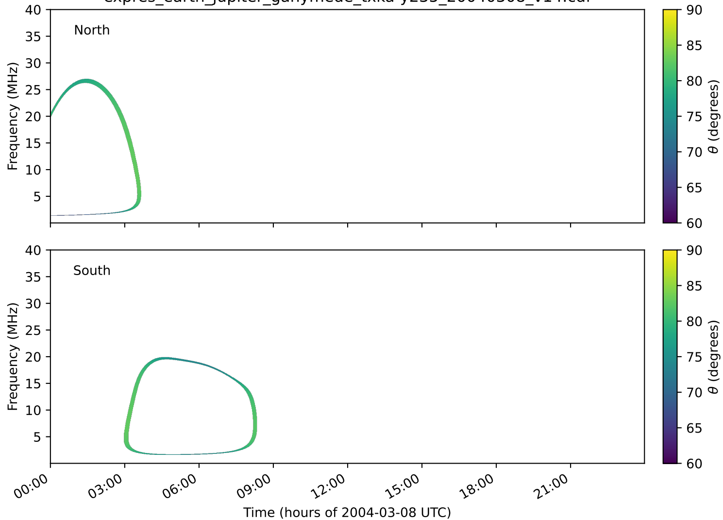
expres_earth_jupiter_ganymede_txka-y235_20040308_v14.cdf
