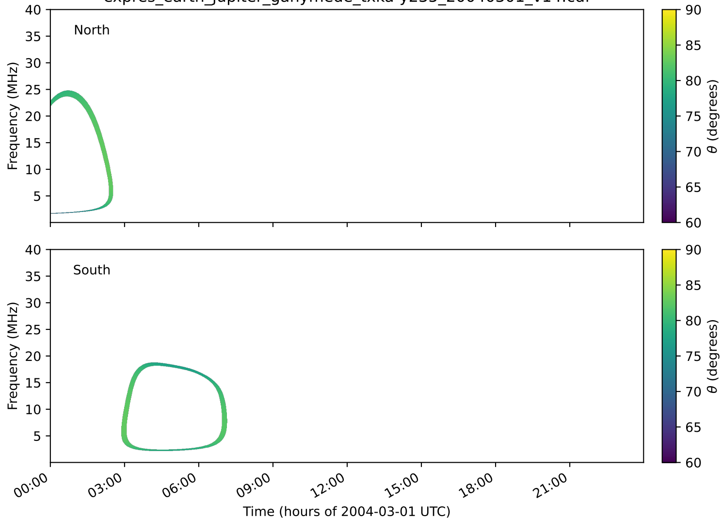
expres_earth_jupiter_ganymede_txka-y235_20040301_v14.cdf
