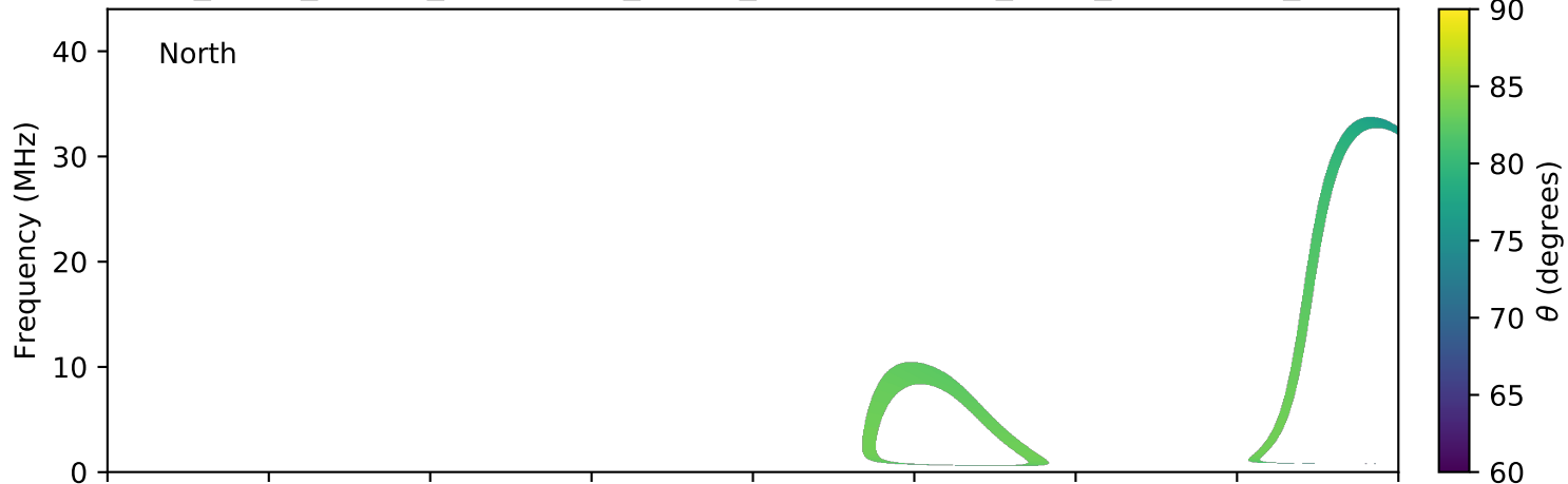
expres_earth_jupiter_ganymede_jrm09_lossc-wid1deg_3kev_20040326_v11.cdf
