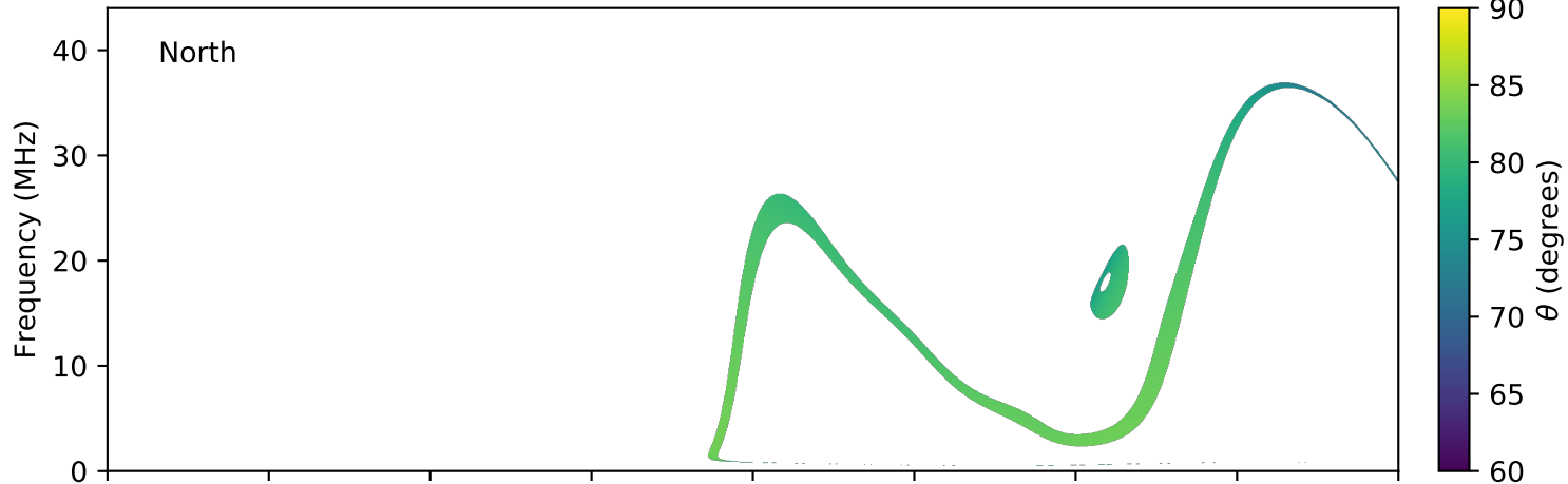
expres_earth_jupiter_ganymede_jrm09_lossc-wid1deg_3kev_20040312_v11.cdf
