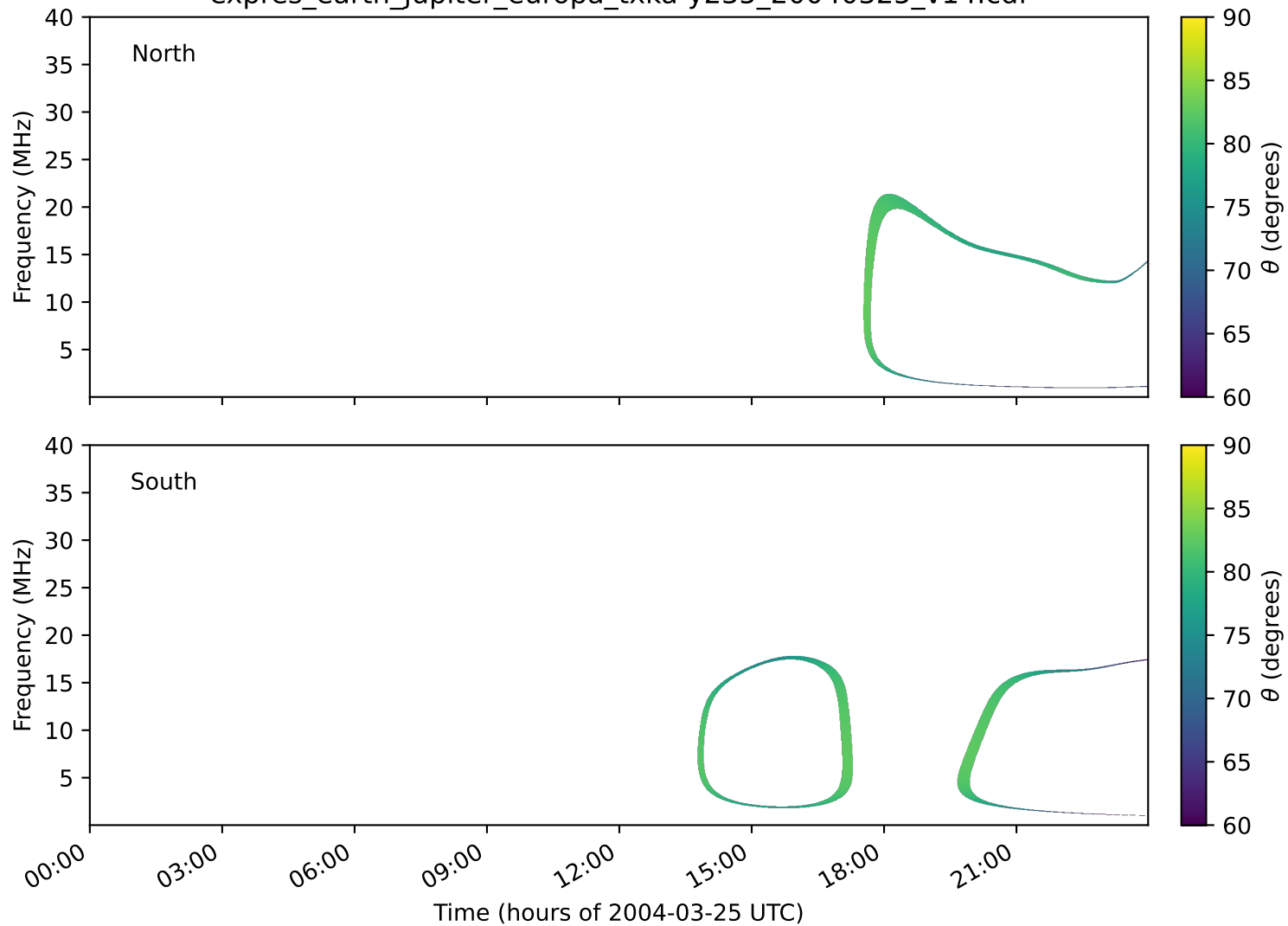
expres_earth_jupiter_europa_txka-y235_20040325_v14.cdf
