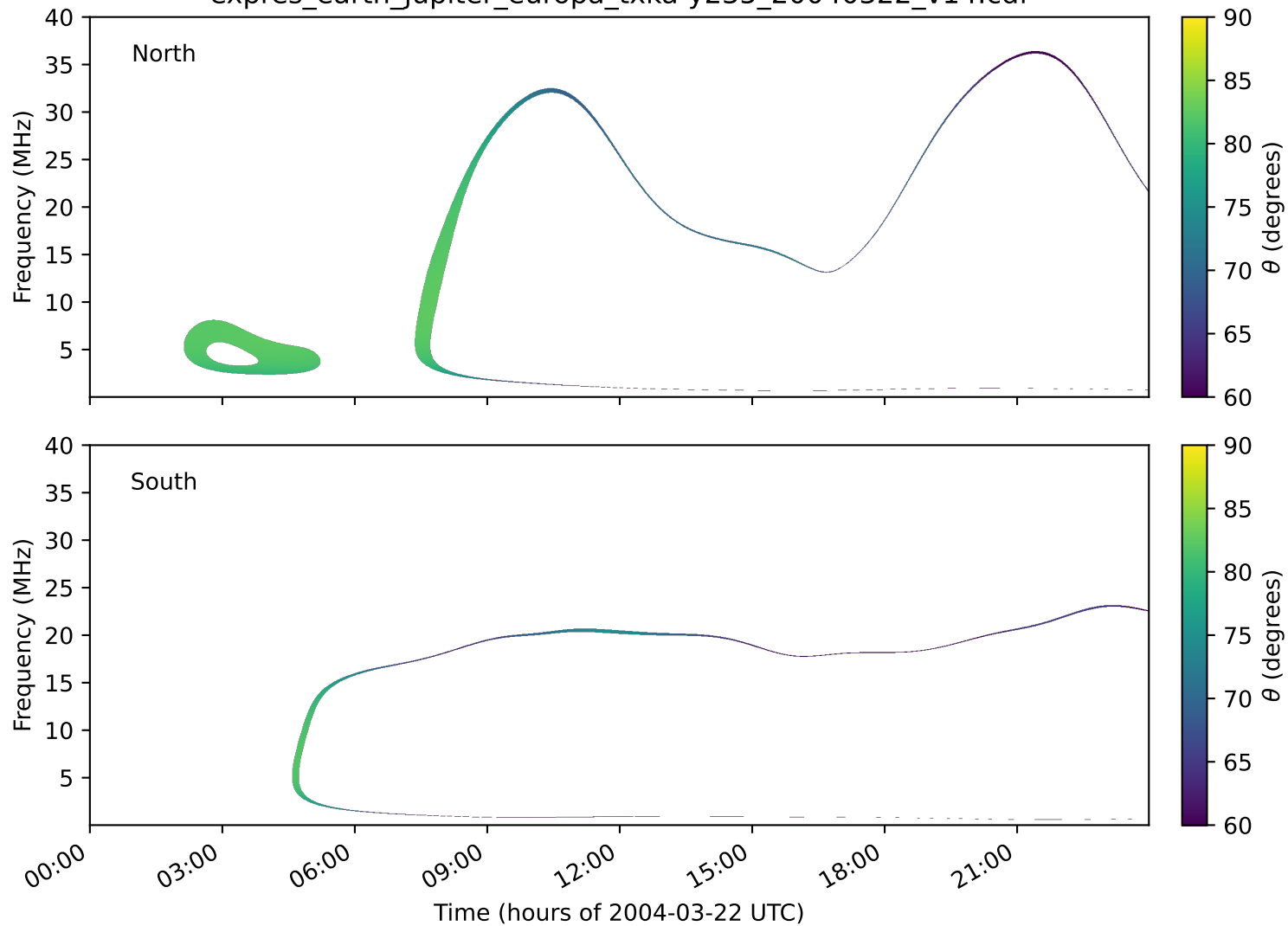
expres_earth_jupiter_europa_txka-y235_20040322_v14.cdf
