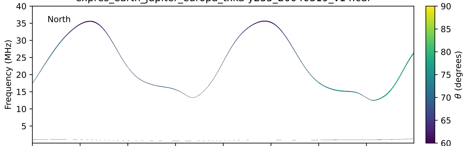
expres_earth_jupiter_europa_txka-y235_20040319_v14.cdf
