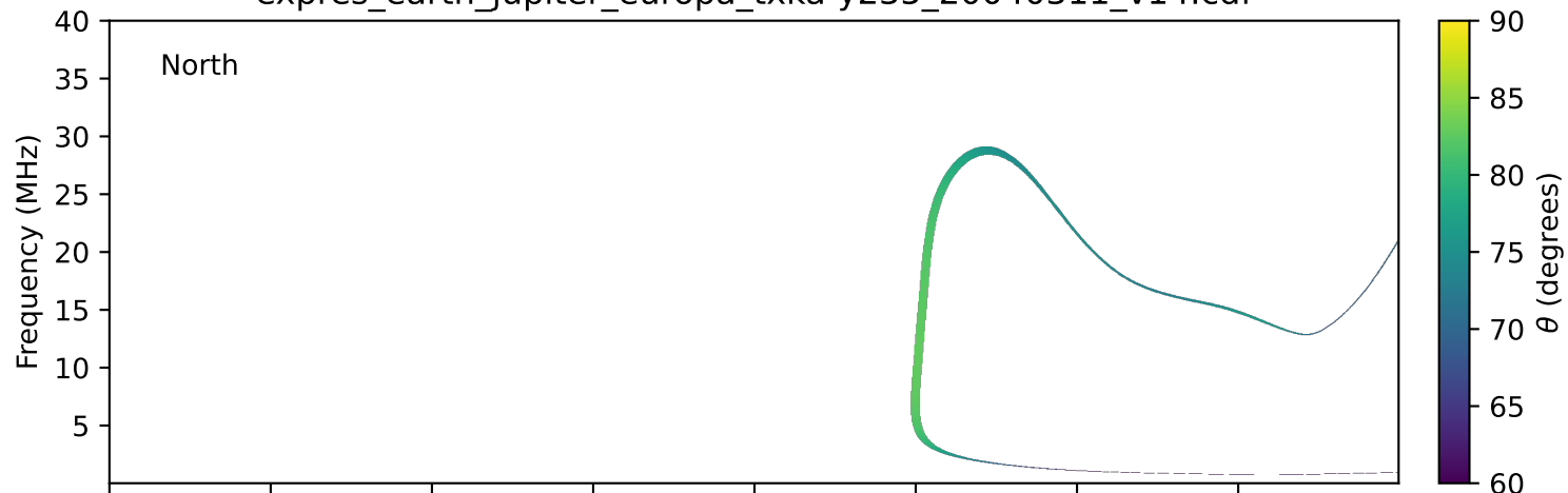
expres_earth_jupiter_europa_txka-y235_20040311_v14.cdf
