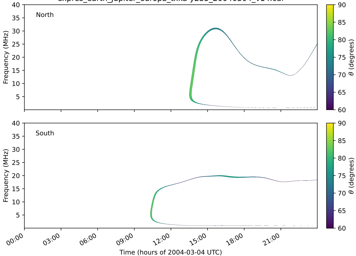
expres_earth_jupiter_europa_txka-y235_20040304_v14.cdf
