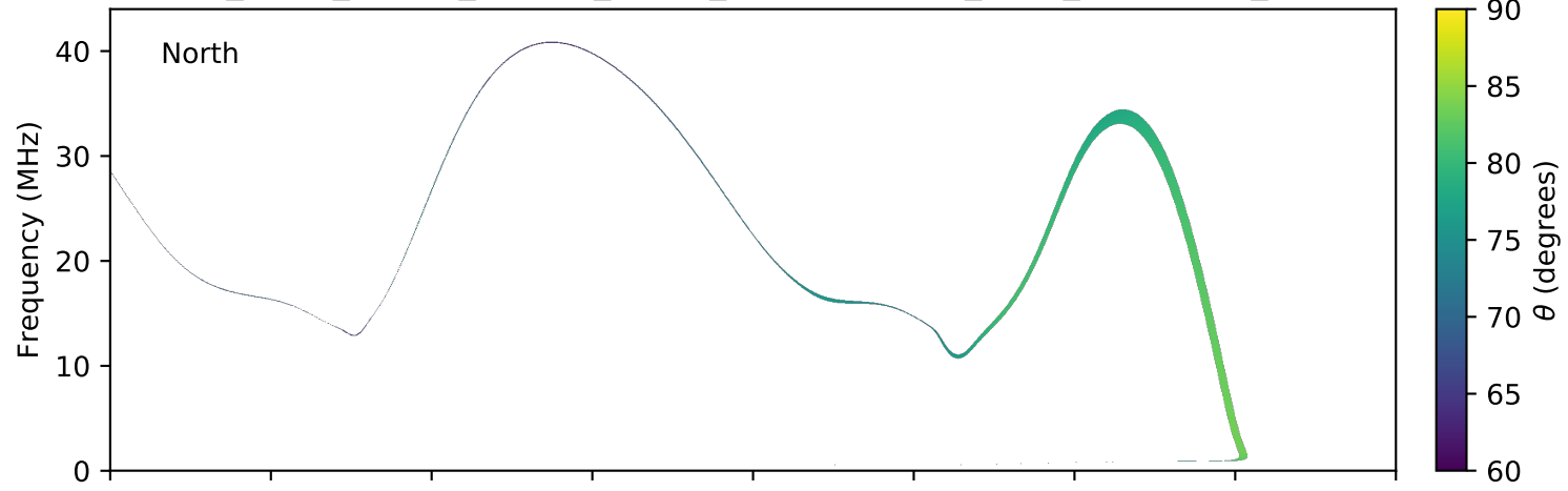
expres_earth_jupiter_europa_jrm09_lossc-wid1deg_3kev_20040330_v11.cdf
