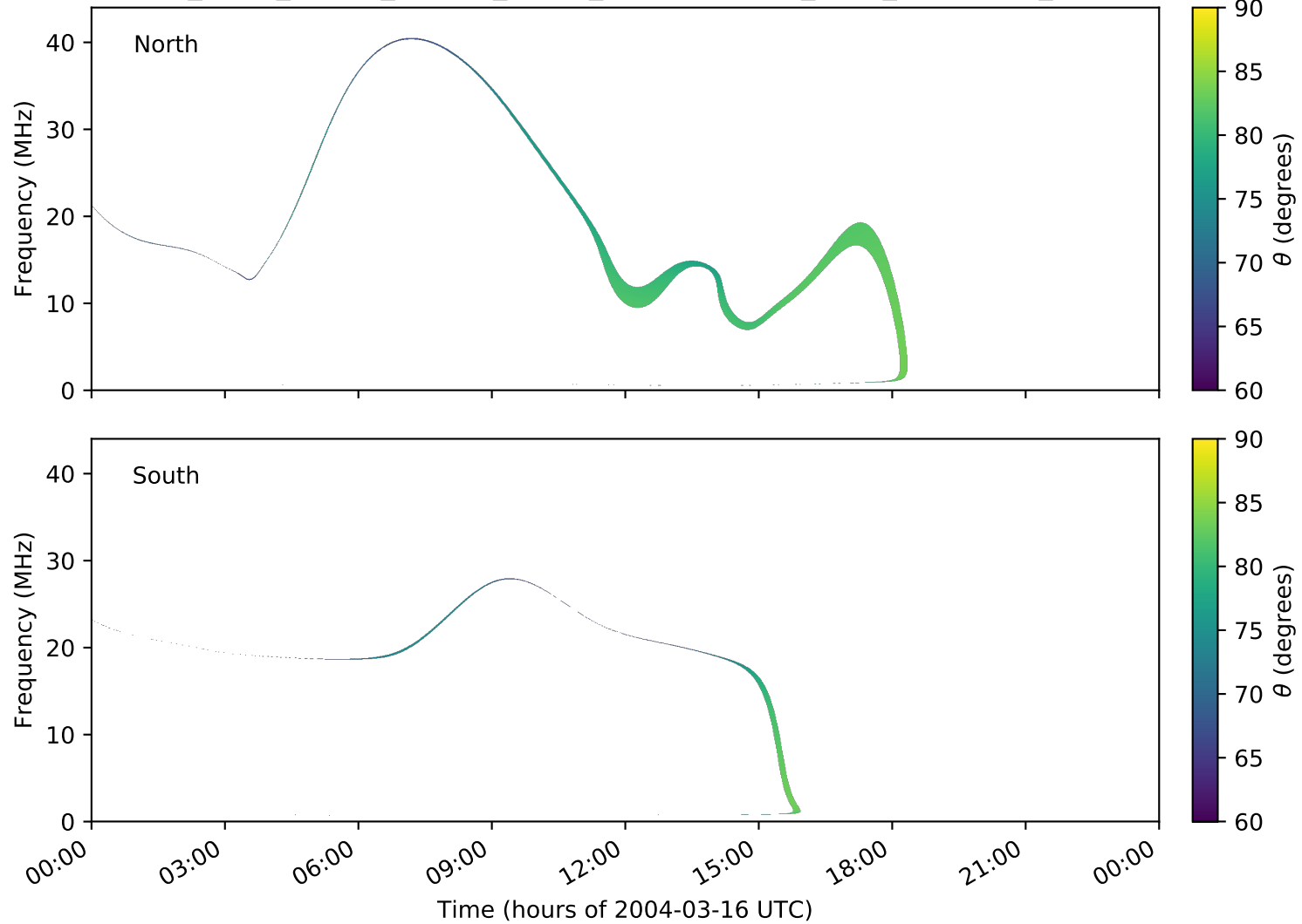
expres_earth_jupiter_europa_jrm09_lossc-wid1deg_3kev_20040316_v11.cdf
