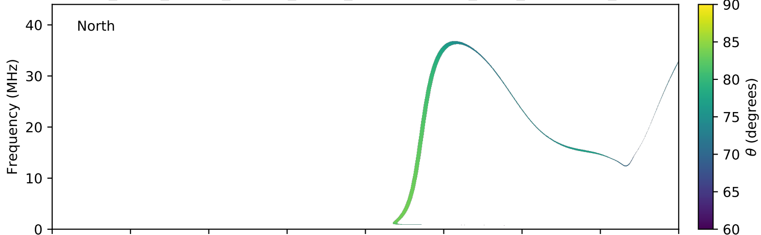
expres_earth_jupiter_europa_jrm09_lossc-wid1deg_3kev_20040304_v11.cdf
