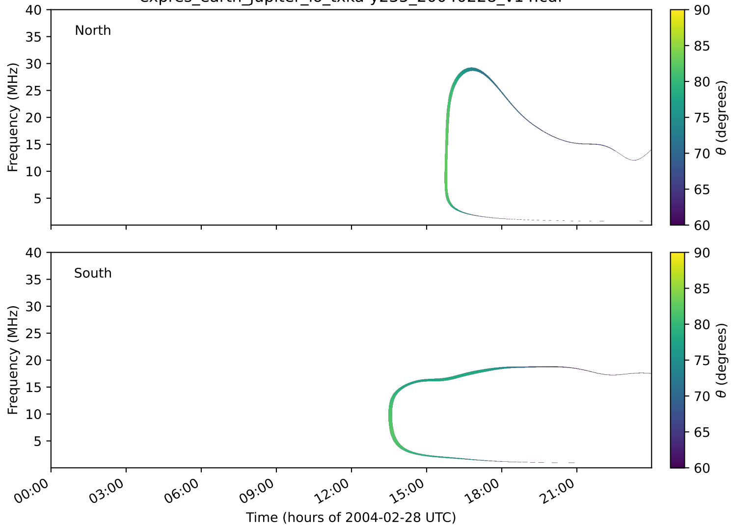
expres_earth_jupiter_io_txka-y235_20040228_v14.cdf
