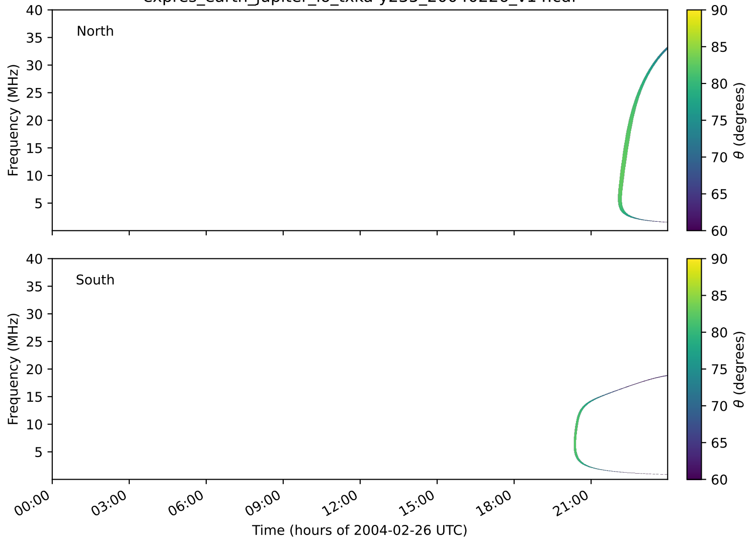
expres_earth_jupiter_io_txka-y235_20040226_v14.cdf
