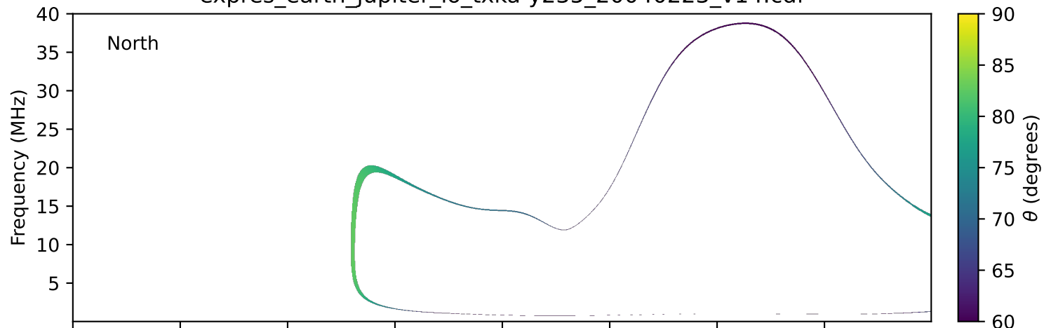
expres_earth_jupiter_io_txka-y235_20040223_v14.cdf
