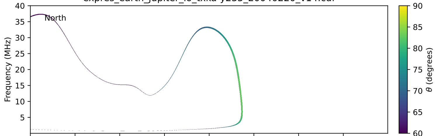
expres_earth_jupiter_io_txka-y235_20040220_v14.cdf
