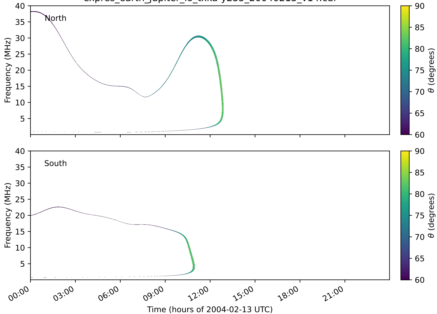
expres_earth_jupiter_io_txka-y235_20040213_v14.cdf
