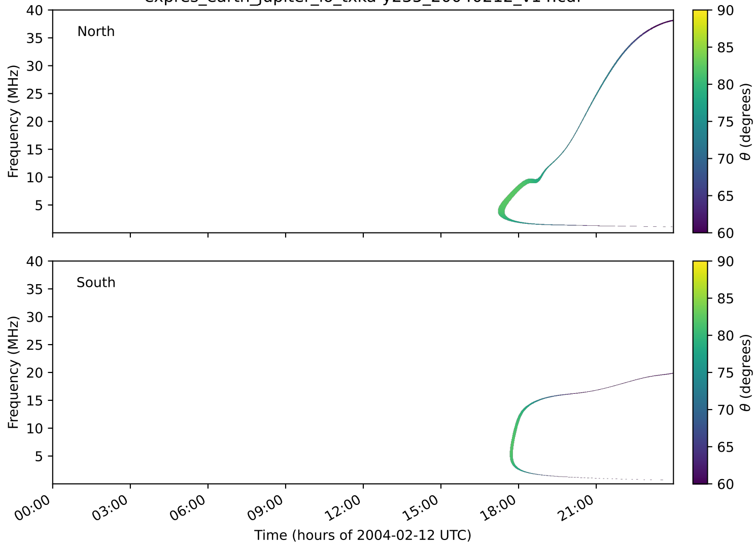
expres_earth_jupiter_io_txka-y235_20040212_v14.cdf
