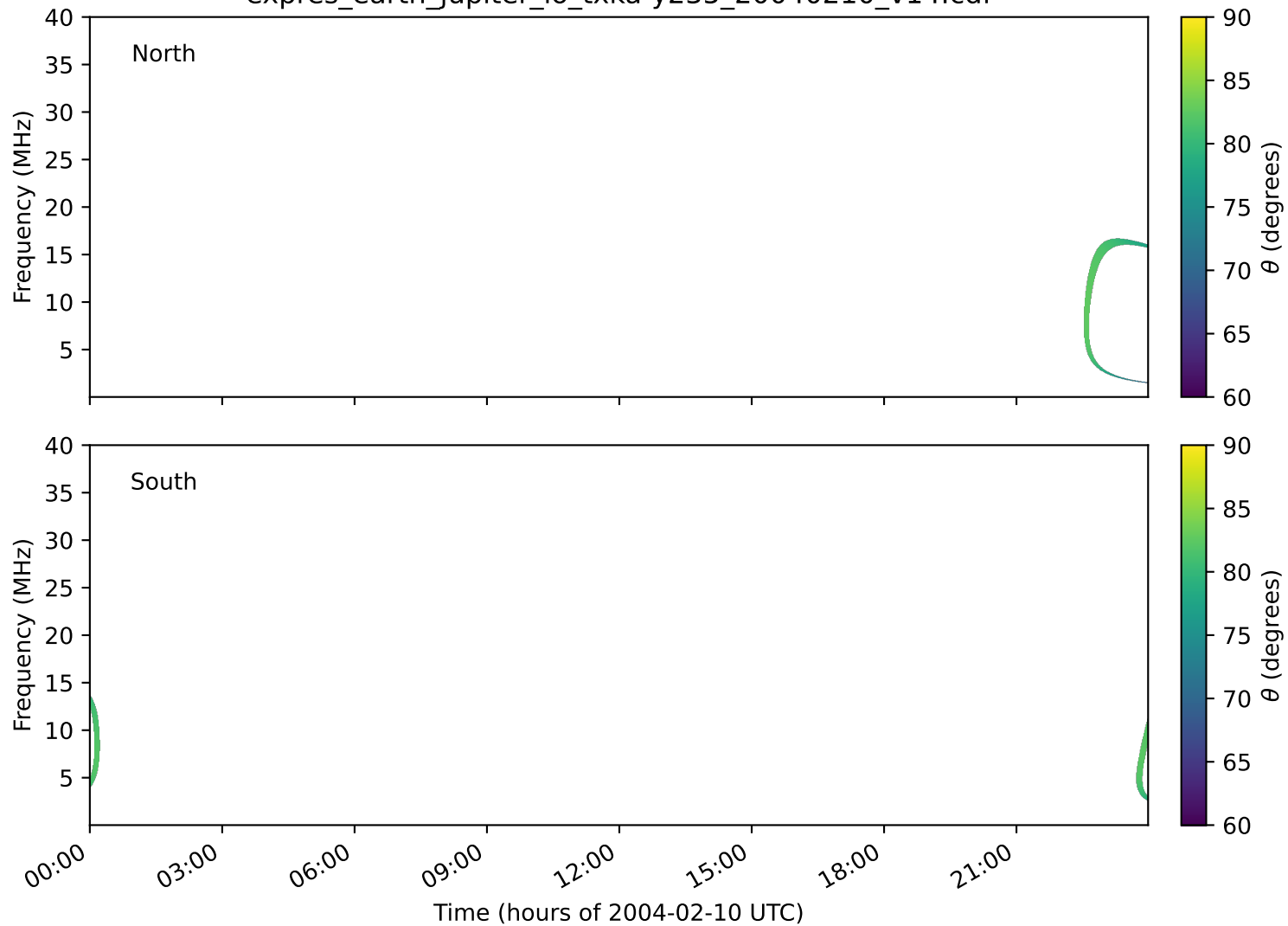
expres_earth_jupiter_io_txka-y235_20040210_v14.cdf
