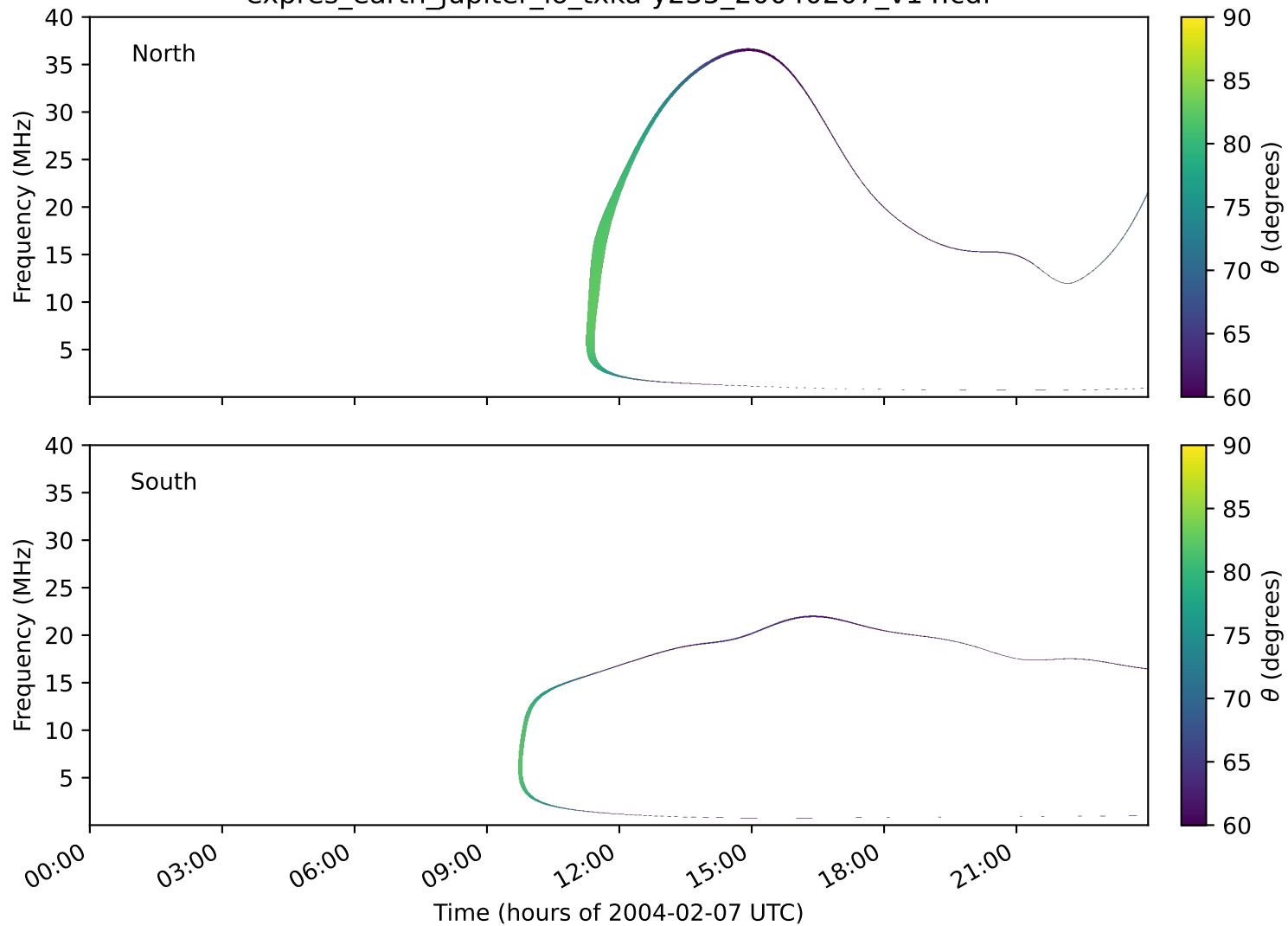
expres_earth_jupiter_io_txka-y235_20040207_v14.cdf
