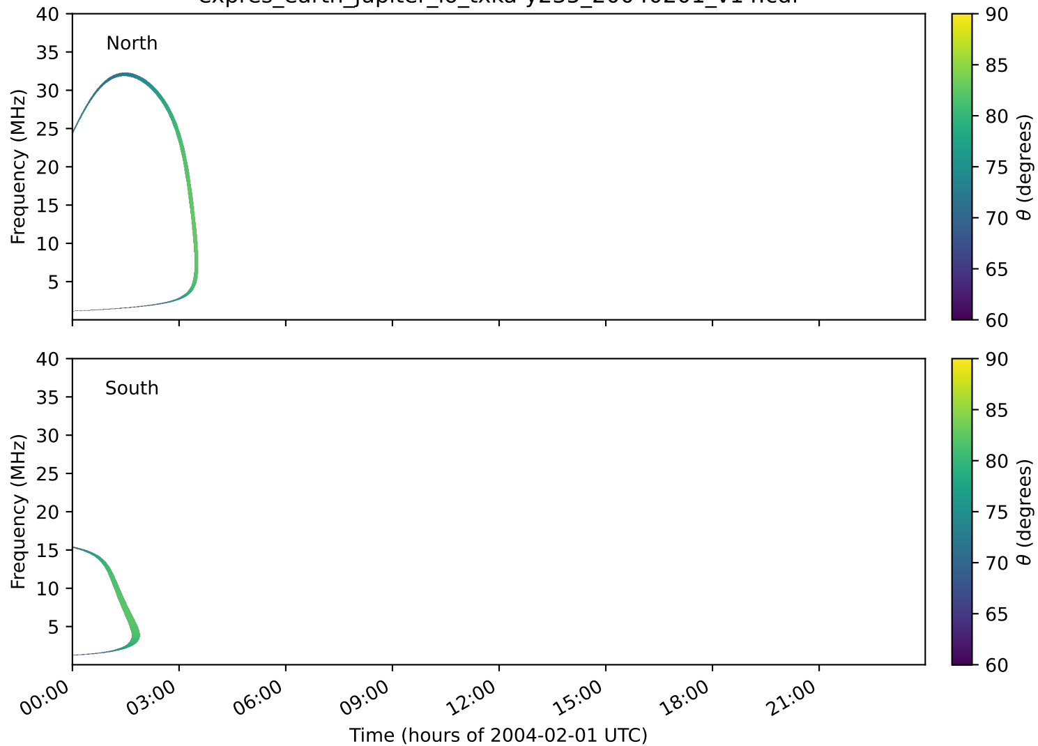
expres_earth_jupiter_io_txka-y235_20040201_v14.cdf
