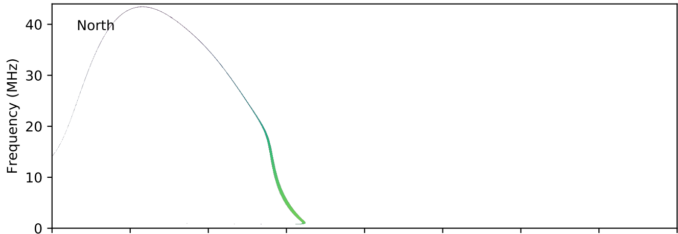
expres_earth_jupiter_io_jrm09_lossc-wid1deg_3kev_20040229_v11.cdf
