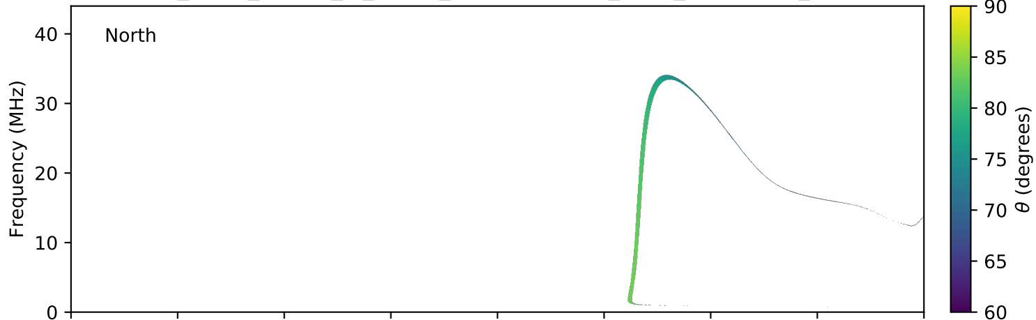
expres_earth_jupiter_io_jrm09_lossc-wid1deg_3kev_20040228_v11.cdf
