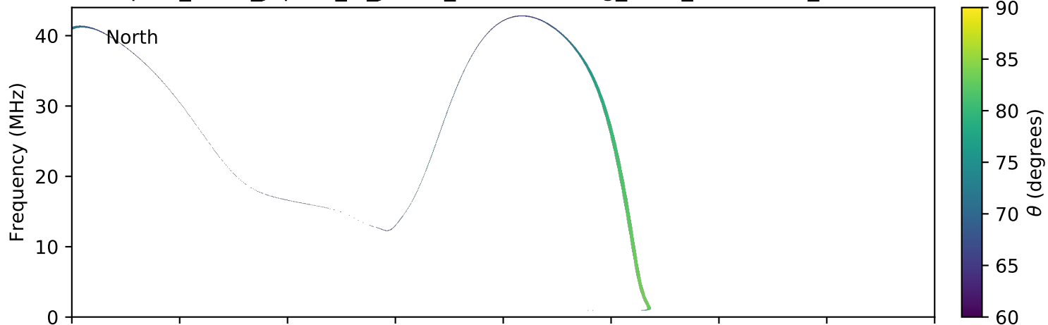
expres_earth_jupiter_io_jrm09_lossc-wid1deg_3kev_20040227_v11.cdf
