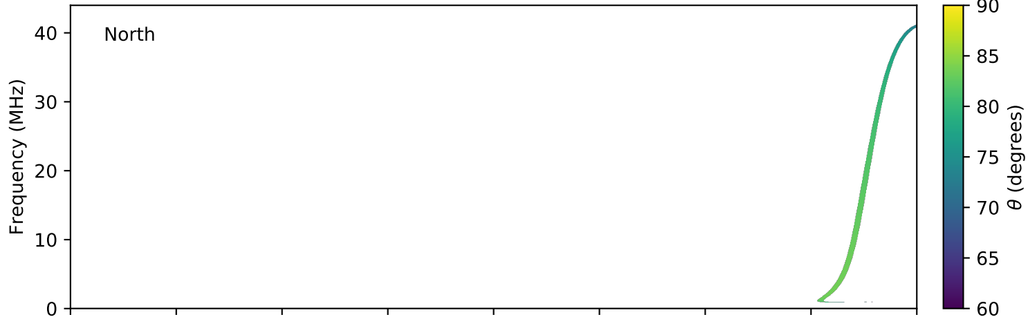
expres_earth_jupiter_io_jrm09_lossc-wid1deg_3kev_20040226_v11.cdf
