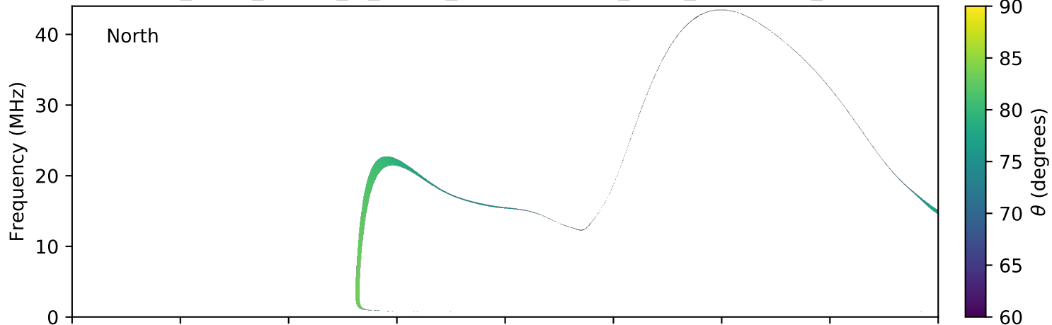
expres_earth_jupiter_io_jrm09_lossc-wid1deg_3kev_20040223_v11.cdf
