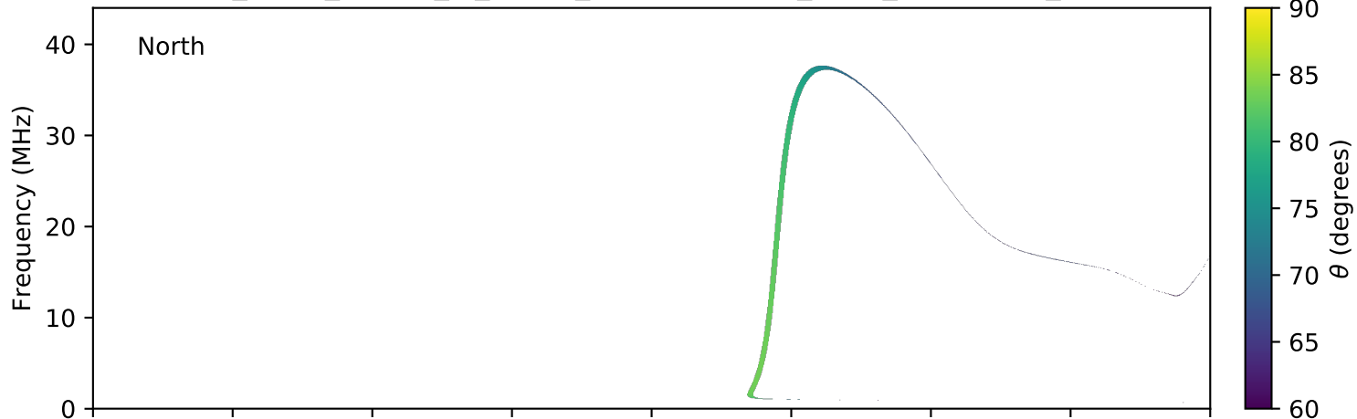
expres_earth_jupiter_io_jrm09_lossc-wid1deg_3kev_20040221_v11.cdf
