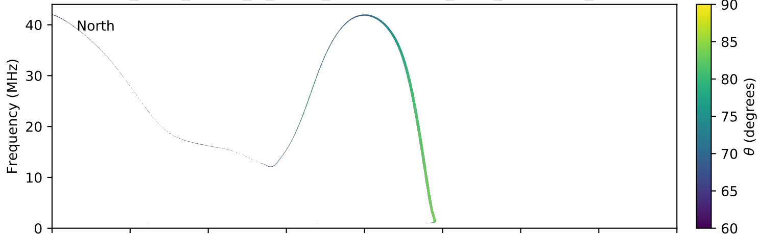
expres_earth_jupiter_io_jrm09_lossc-wid1deg_3kev_20040220_v11.cdf
