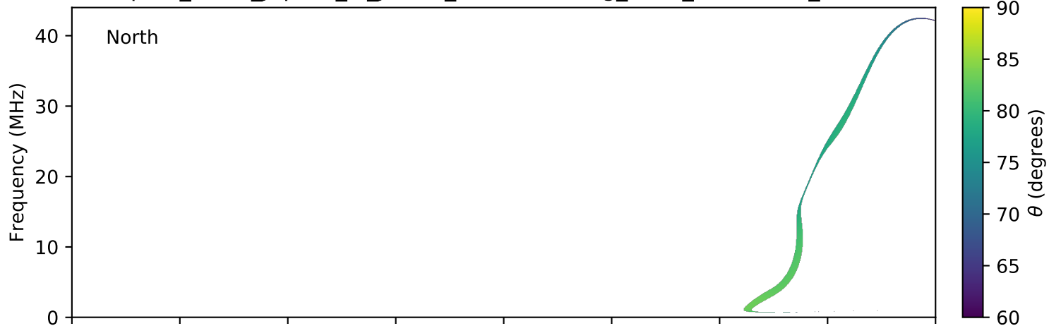
expres_earth_jupiter_io_jrm09_lossc-wid1deg_3kev_20040219_v11.cdf
