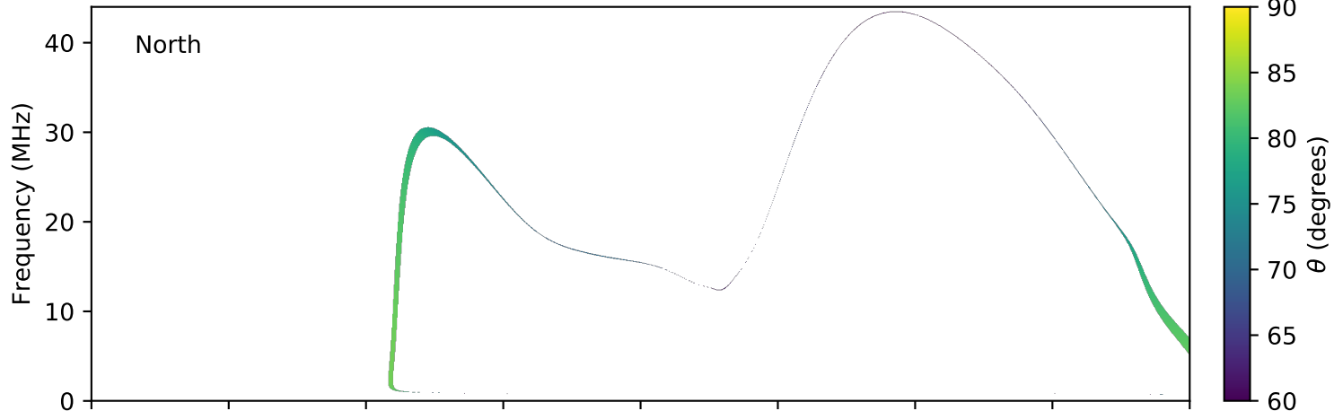
expres_earth_jupiter_io_jrm09_lossc-wid1deg_3kev_20040216_v11.cdf
