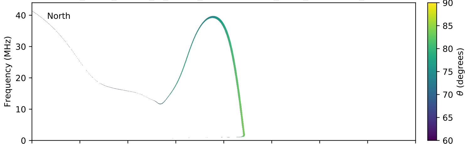
expres_earth_jupiter_io_jrm09_lossc-wid1deg_3kev_20040213_v11.cdf
