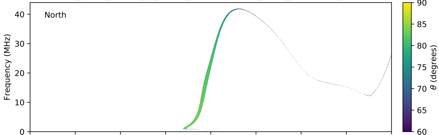
expres_earth_jupiter_io_jrm09_lossc-wid1deg_3kev_20040207_v11.cdf
