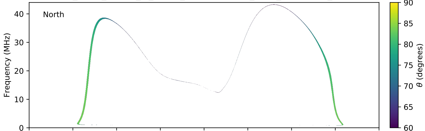
expres_earth_jupiter_io_jrm09_lossc-wid1deg_3kev_20040202_v11.cdf
