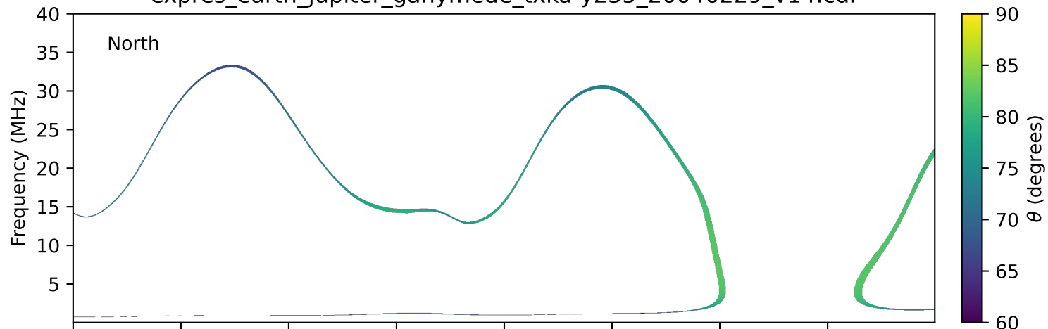
expres_earth_jupiter_ganymede_txka-y235_20040229_v14.cdf
