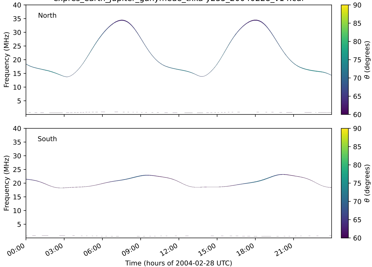
expres_earth_jupiter_ganymede_txka-y235_20040228_v14.cdf
