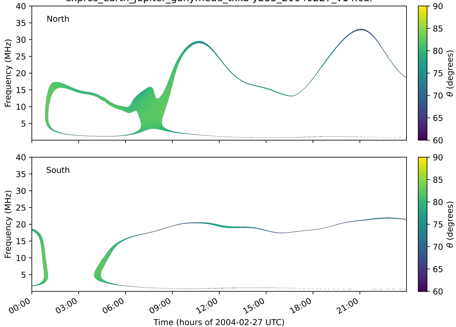
expres_earth_jupiter_ganymede_txka-y235_20040227_v14.cdf
