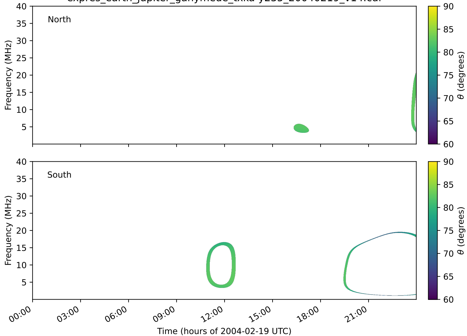
expres_earth_jupiter_ganymede_txka-y235_20040219_v14.cdf
