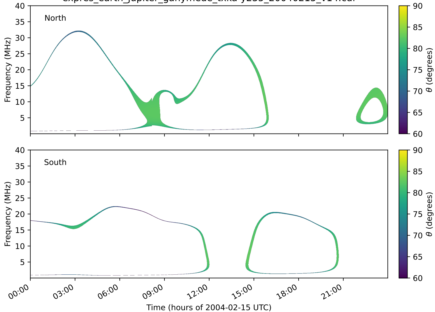
expres_earth_jupiter_ganymede_txka-y235_20040215_v14.cdf
