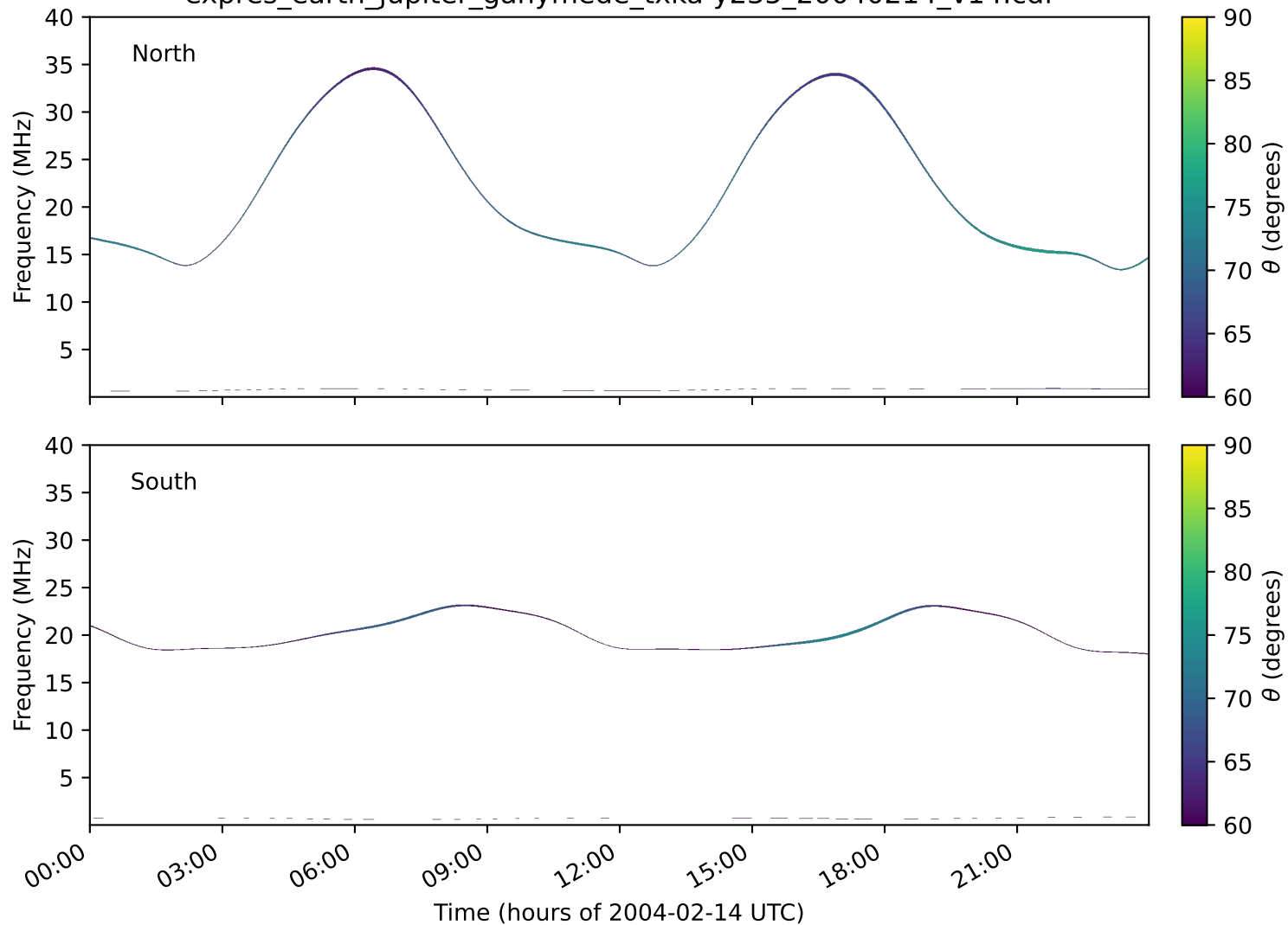
expres_earth_jupiter_ganymede_txka-y235_20040214_v14.cdf
