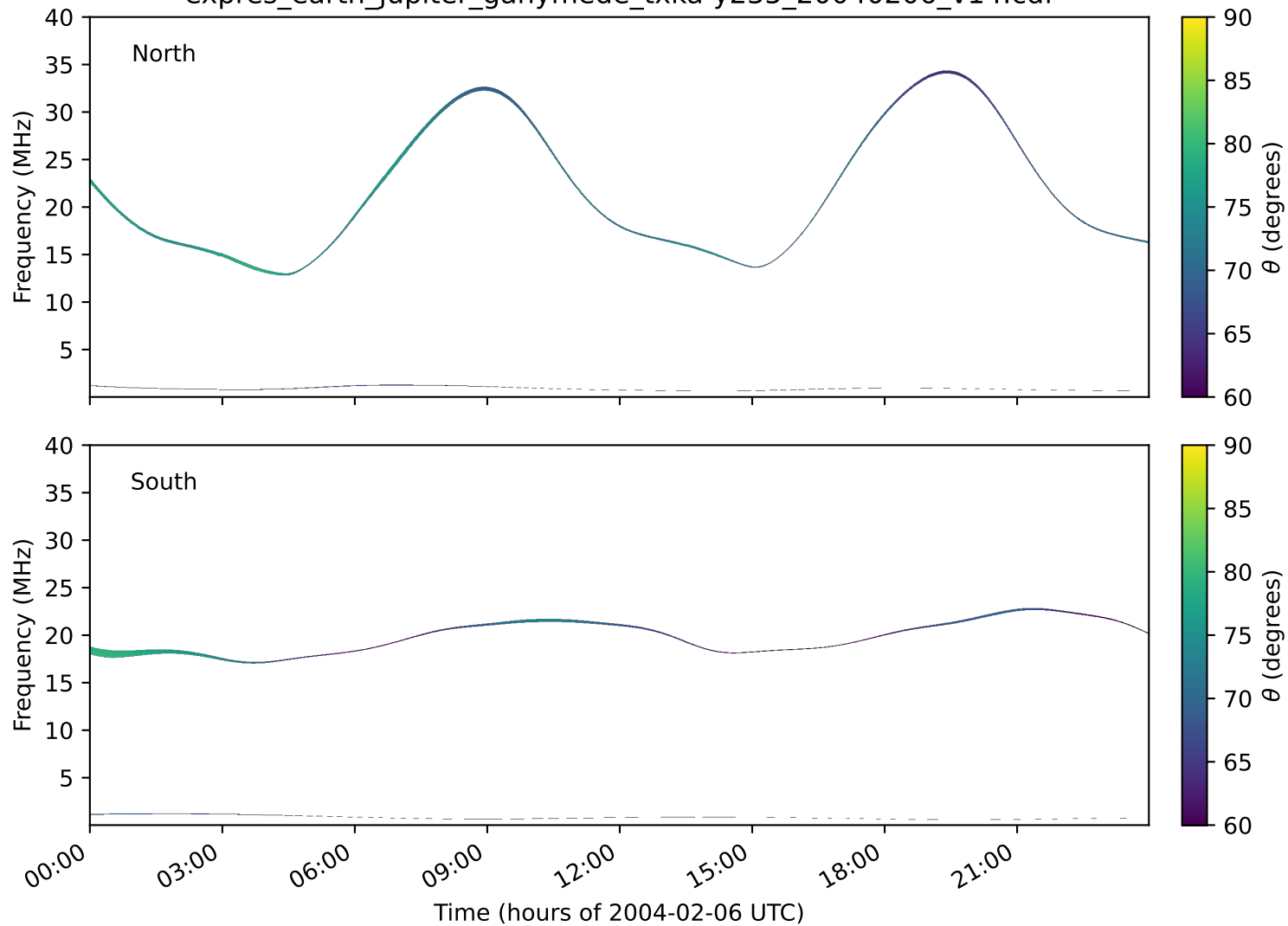
expres_earth_jupiter_ganymede_txka-y235_20040206_v14.cdf
