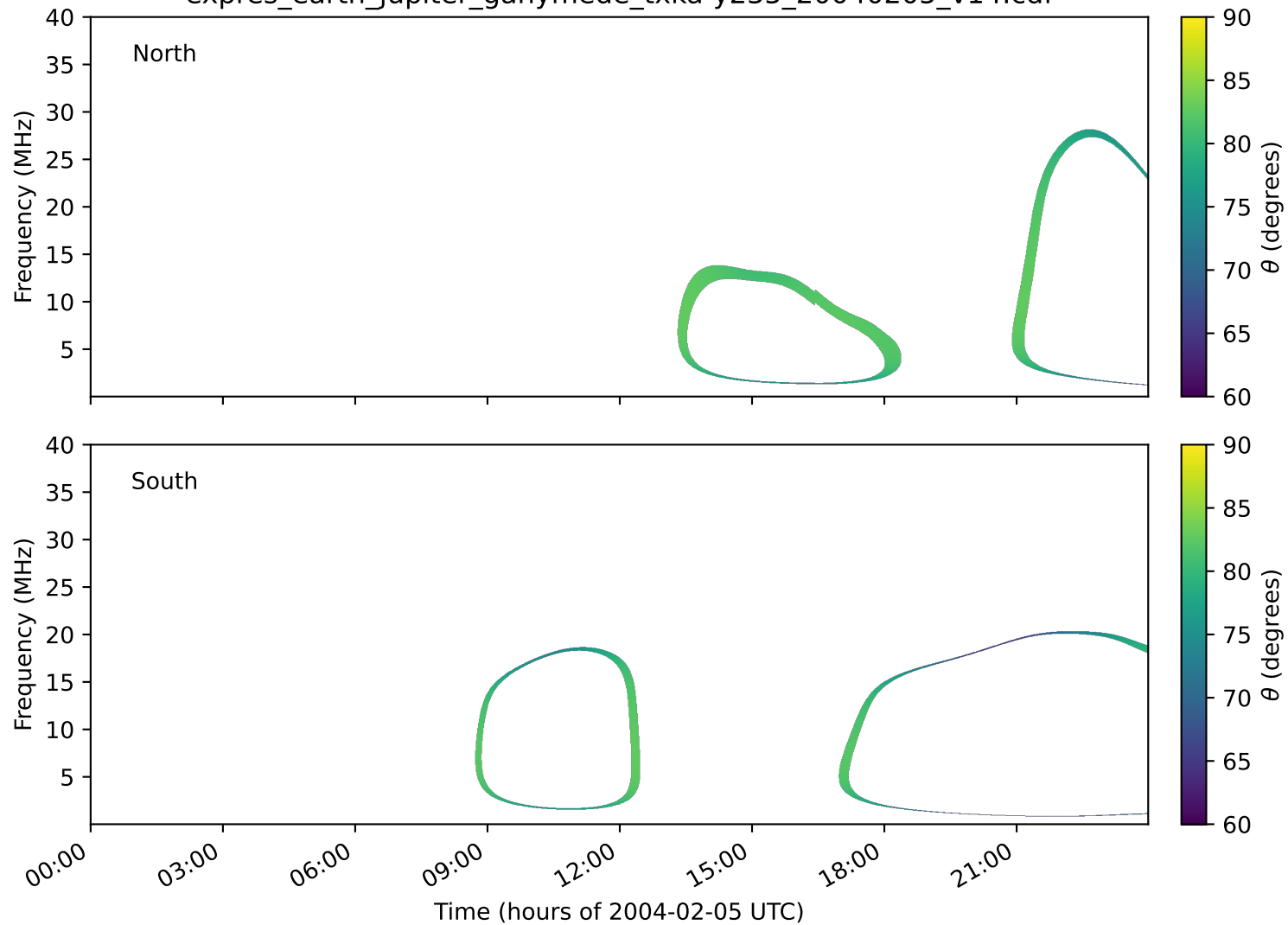
expres_earth_jupiter_ganymede_txka-y235_20040205_v14.cdf
