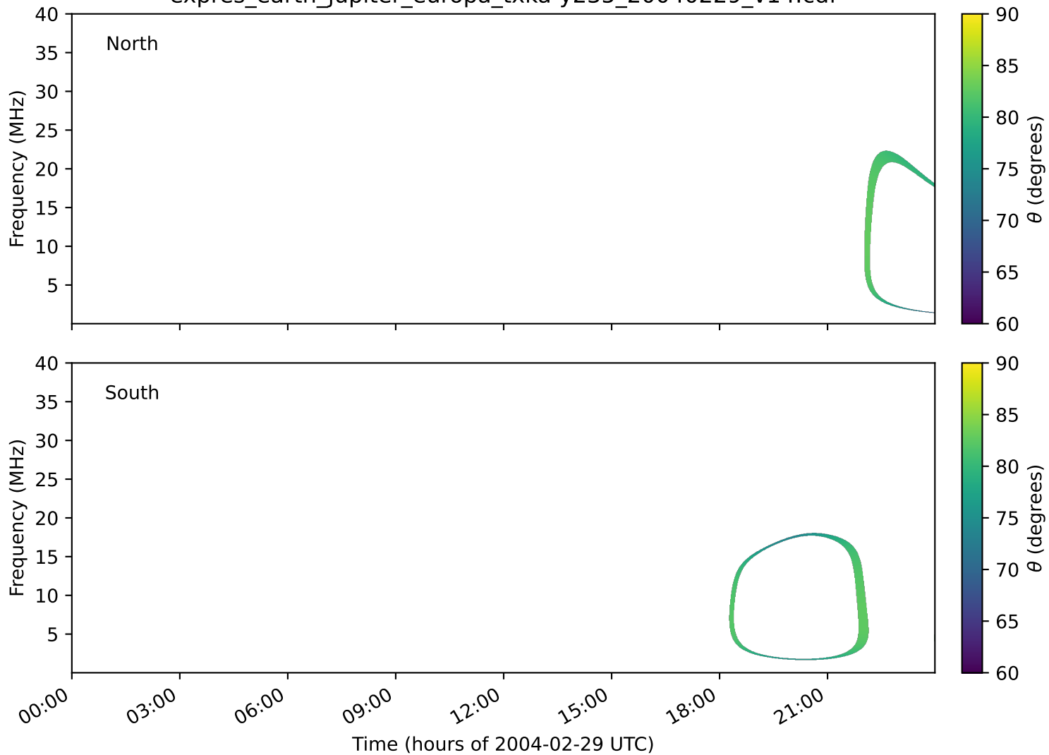
expres_earth_jupiter_europa_txka-y235_20040229_v14.cdf
