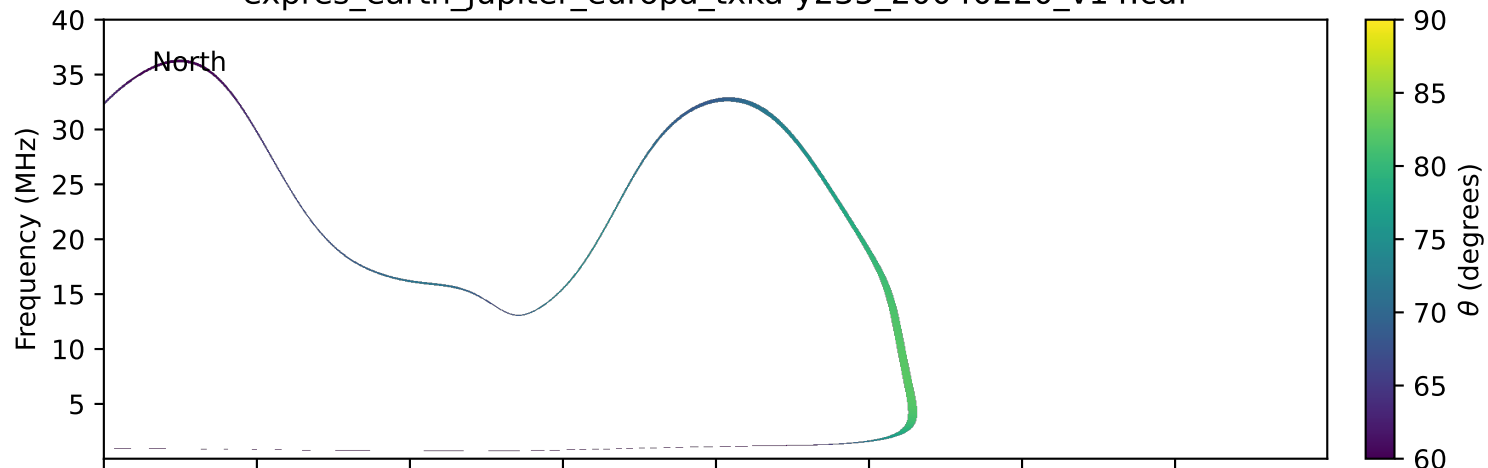
expres_earth_jupiter_europa_txka-y235_20040220_v14.cdf
