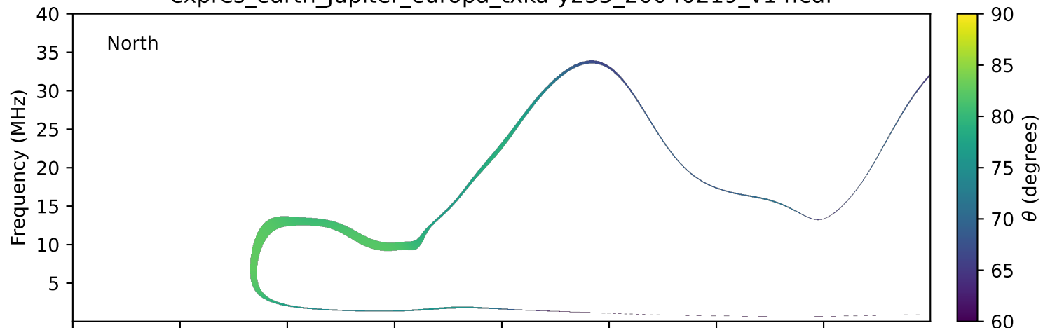
expres_earth_jupiter_europa_txka-y235_20040219_v14.cdf
