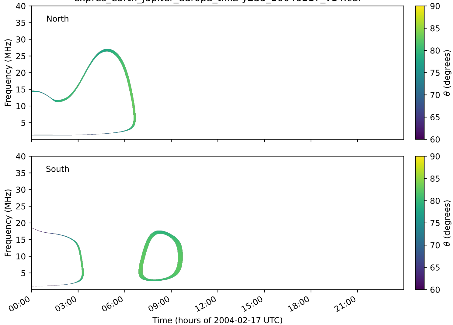
expres_earth_jupiter_europa_txka-y235_20040217_v14.cdf
