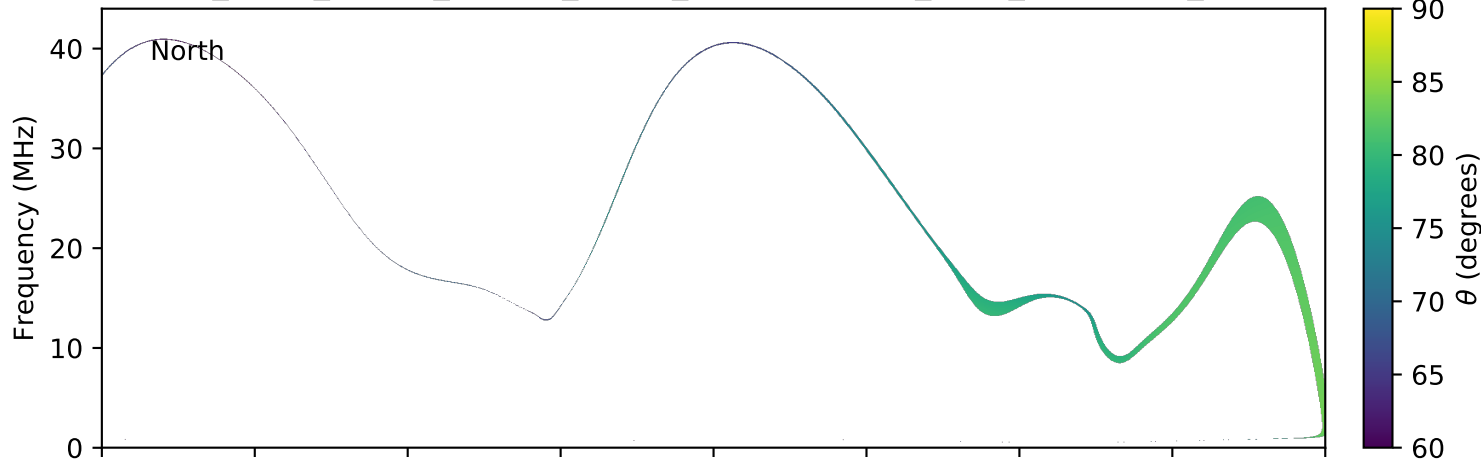
expres_earth_jupiter_europa_jrm09_lossc-wid1deg_3kev_20040227_v11.cdf
