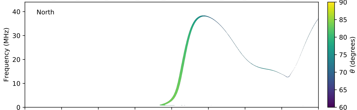
expres_earth_jupiter_europa_jrm09_lossc-wid1deg_3kev_20040226_v11.cdf
