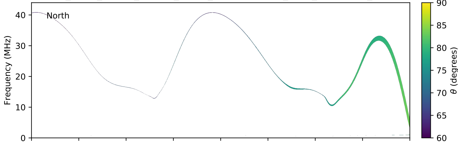
expres_earth_jupiter_europa_jrm09_lossc-wid1deg_3kev_20040220_v11.cdf
