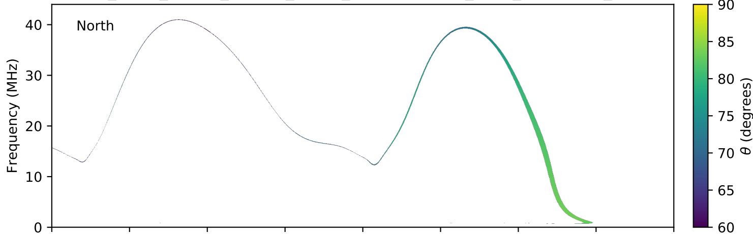
expres_earth_jupiter_europa_jrm09_lossc-wid1deg_3kev_20040217_v11.cdf
